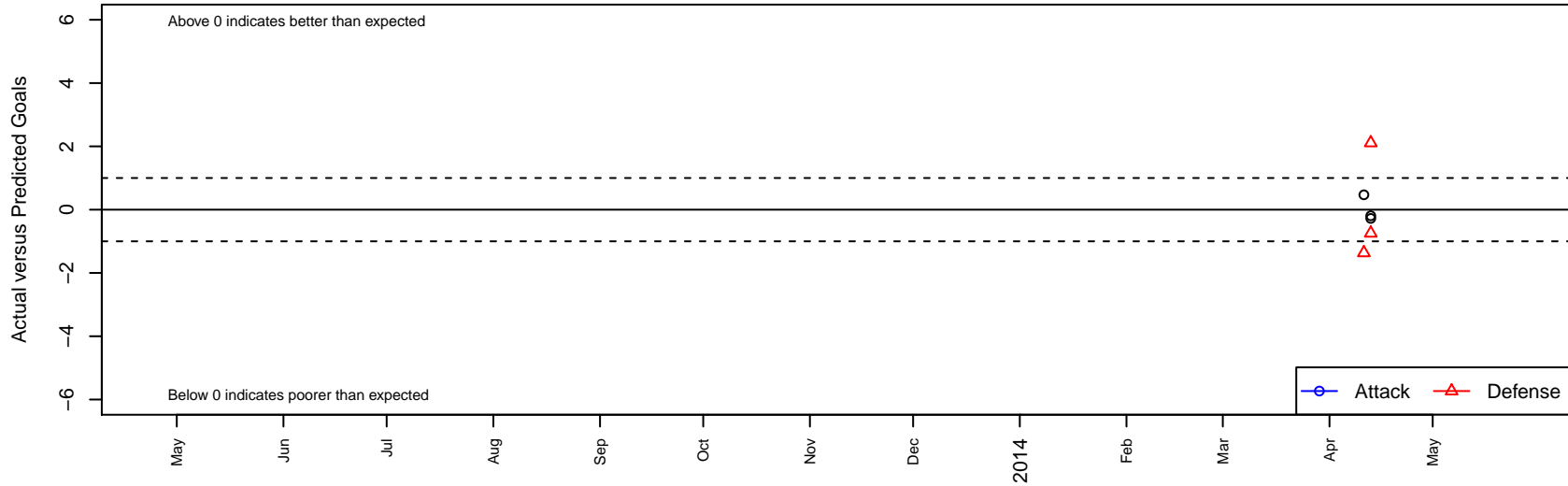
Spokane Foxes –Unk 3 G00 Dots are actual minus expected GF (blue circles) and GA (red triangles). Blue line is smoothed change in attack strength. Red is smoothed change in defense strength.
